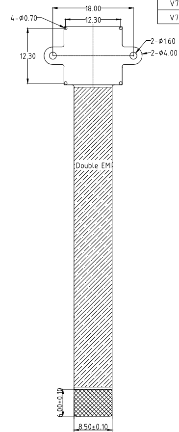
BOTTOM VIEW
