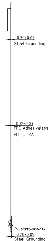
SIDE VIEW
