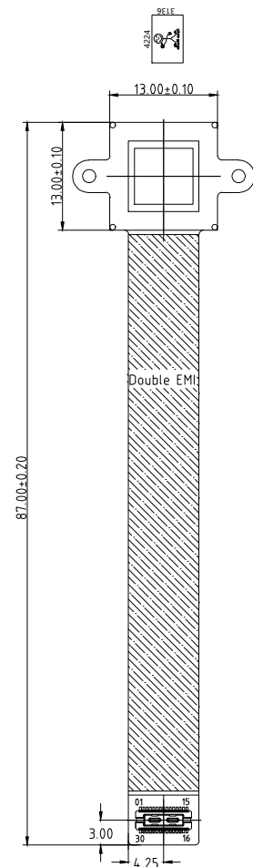
TOP VIEW
